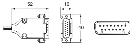
15-way D-type plug (Termination code D, L)
